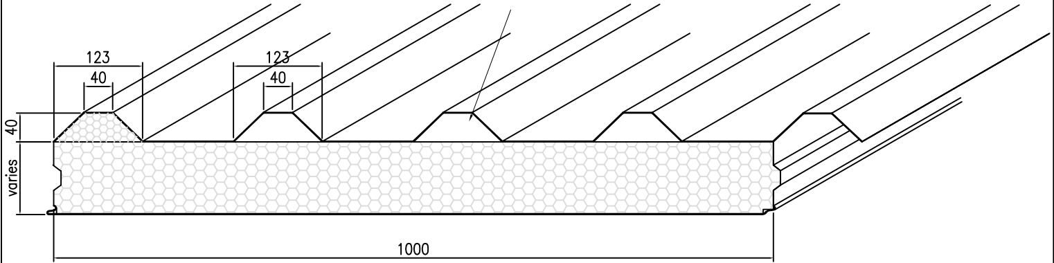
DPR ROOF PANEL WITHOUT CROWN INSERT
