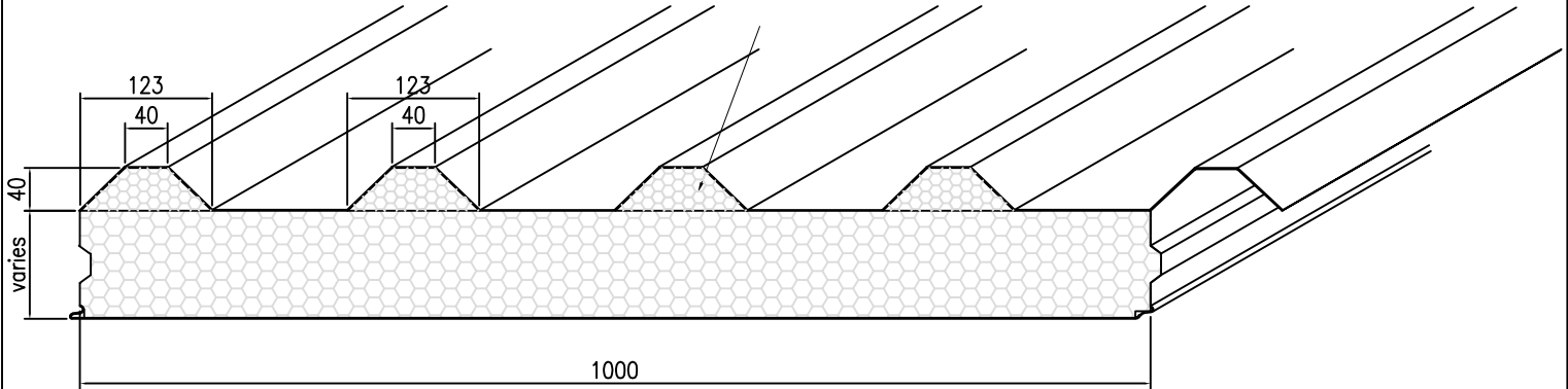
DPR ROOF PANEL WITH CROWN INSERT
